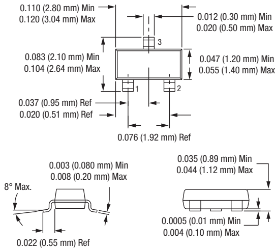
Figure 12. SOT-23 Package Dimensions
